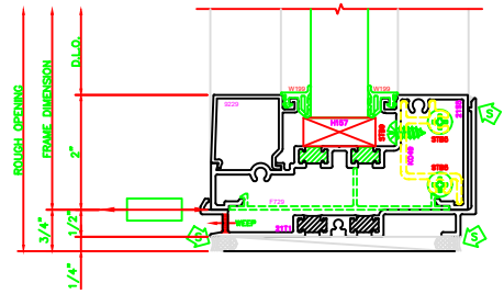
203 O.G. SILL SERIES: 403X - 2" X 4 1/2" SHEARBLOCK
